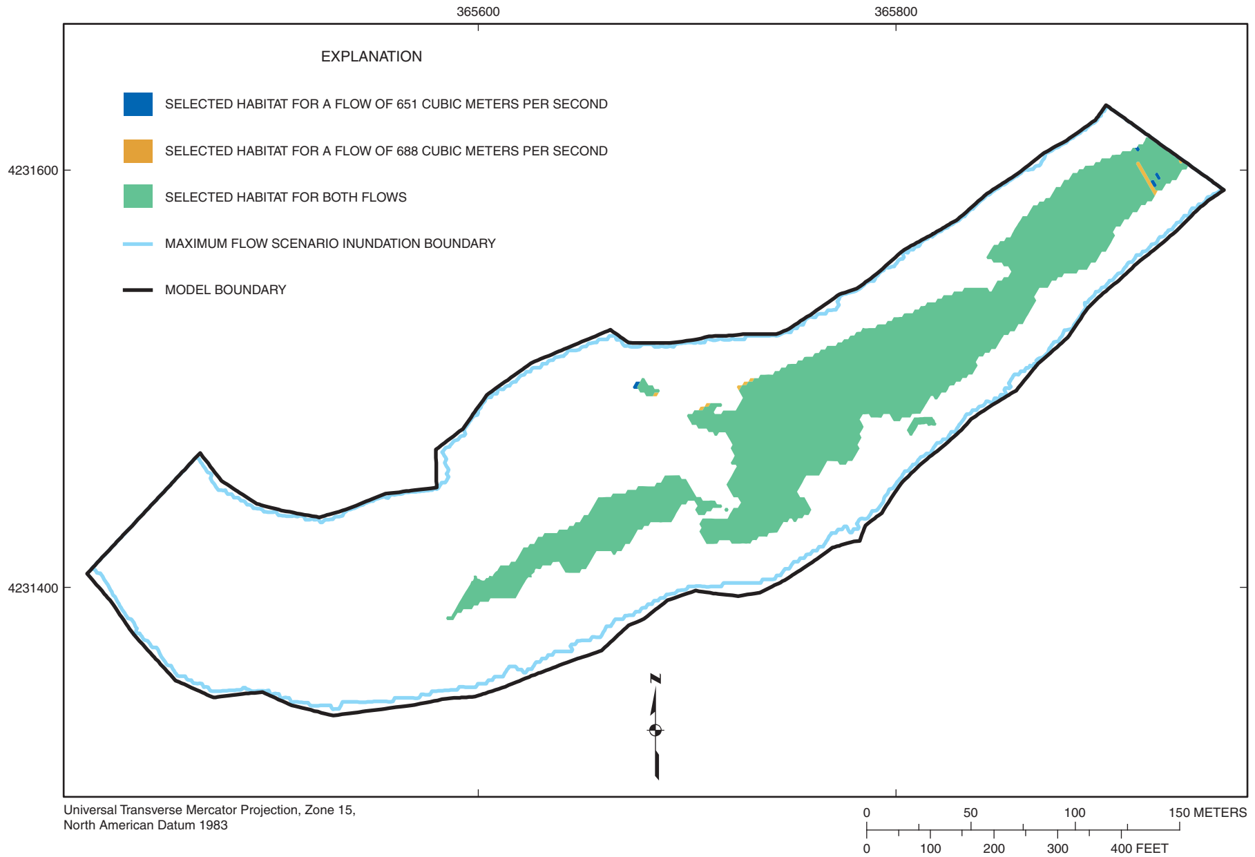
Figure 4-45. Selected habitat area distribution for habitat category 7 (paddlefish) at flows of 651 and 688 cubic meters per second at Marais des Cygnes River site MDC2.
